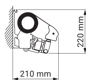
Wandmontage
