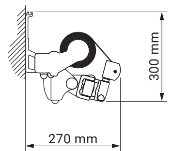
Wandmontage
