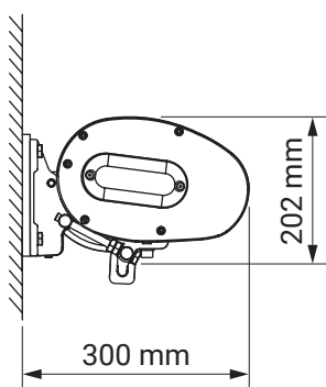
Wandmontage
