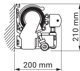
Wandmontage
