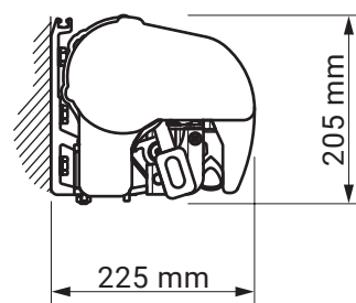
Wandmontage
